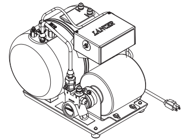
Carbonator Power supply: 115 V; 75 VA Fittings: 1/4" barbed CO2 3/8" barbed water NSF, UL Approved
